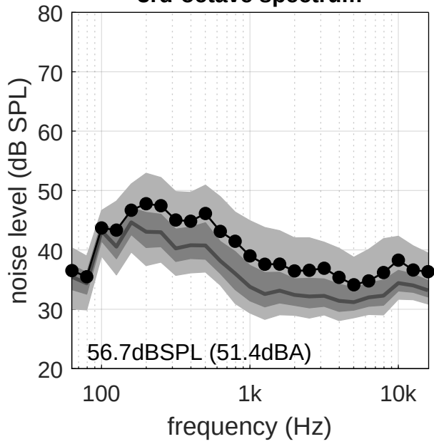
3rd-octave spectrum
